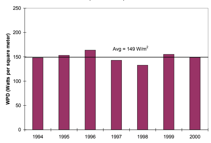
Annual Wind Power Density at 10 m (1994 to 2000)
