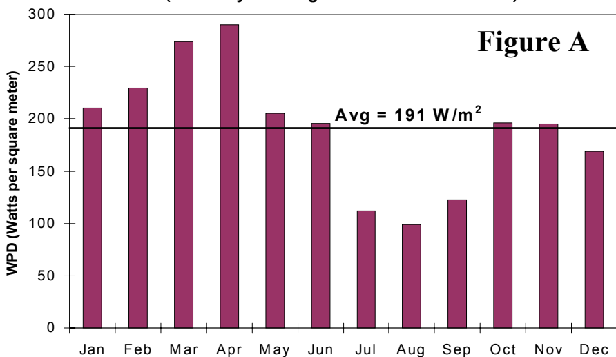
Monthly Wind Power Density at 10-meters (Monthly Averages over 1994 to 2002)
