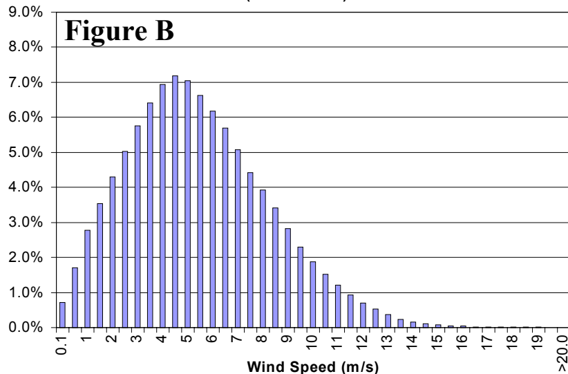
Frequency Distribution of Winds (1994 to 2002)
