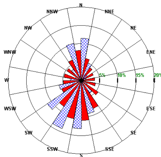
Good Annual Rose Plot ■ Percent of Total Time ■ Percent of Total Wind Energy
