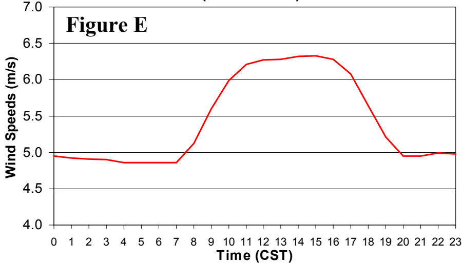
Annual Diurnal Wind Speeds at 10-meters (1994 - 2002)
