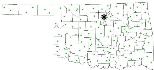
Monthly Wind Power Density at 10 m (Monthly Averages over 1994 to 2002)
