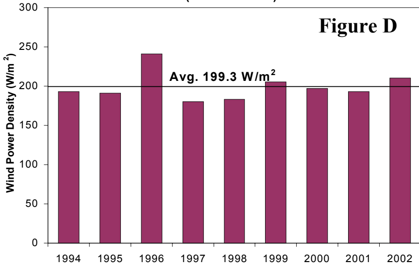
Annual Wind Power Density at 10-meters (1994 to 2002)
