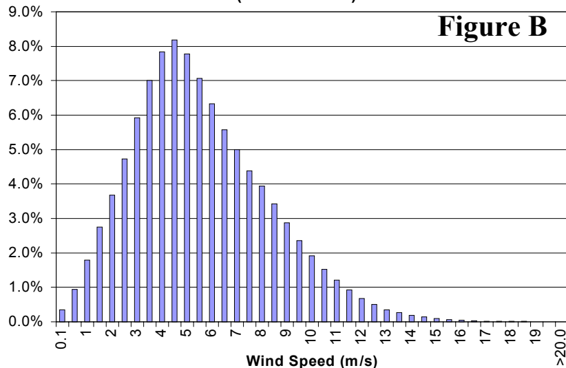
Frequency Distribution of Winds at 10-meters (1994 to 2002)
